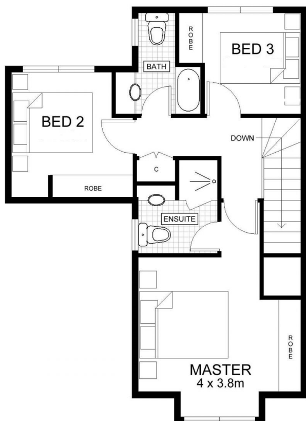
UPPER LEVEL
