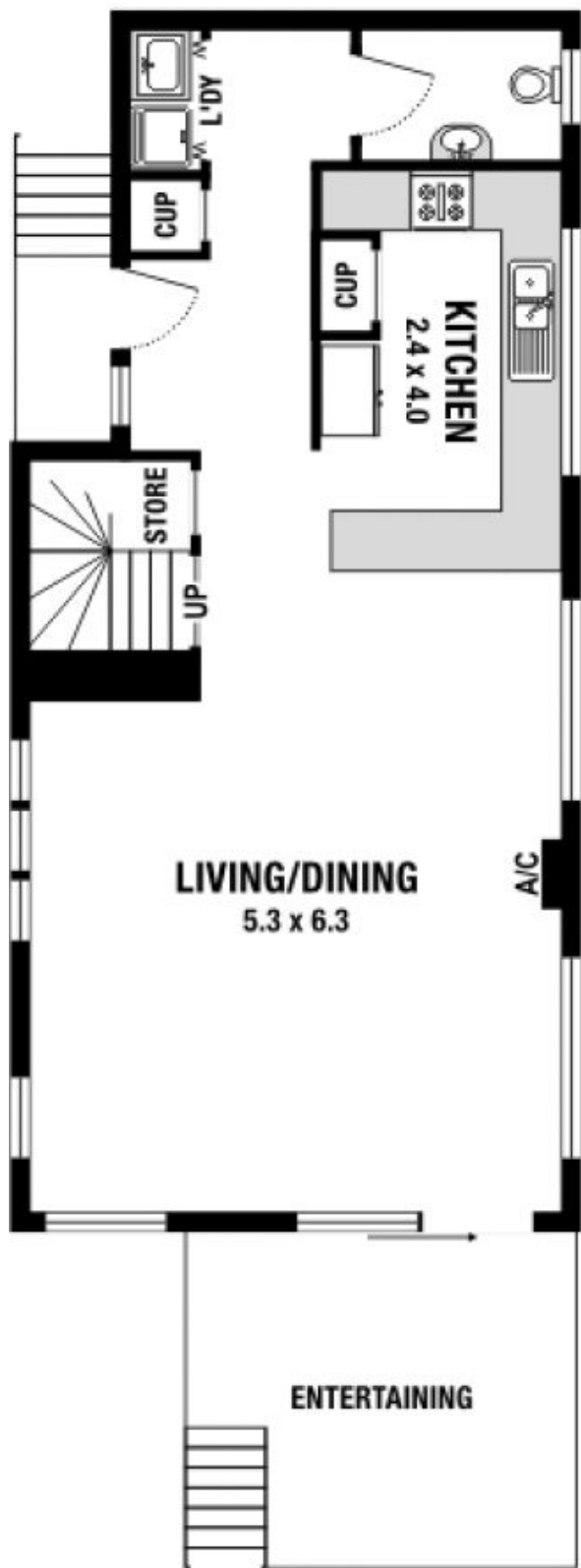
GROUND FLOOR
